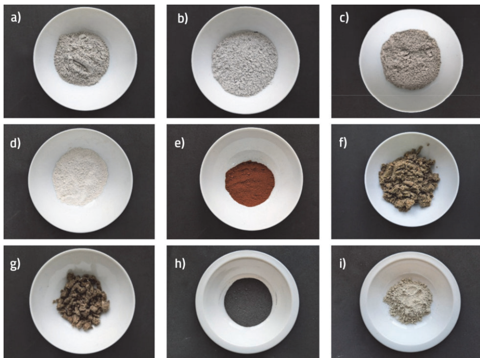
Figure 1. a) Biomass ash 1; b) Biomass ash 2; c) Biomass ash 3; d) Concrete powder; e) Red mud; f) Raw olive pomace; g) Raw paper sludge; h) Olive pomace ash; i) Paper sludge ash
